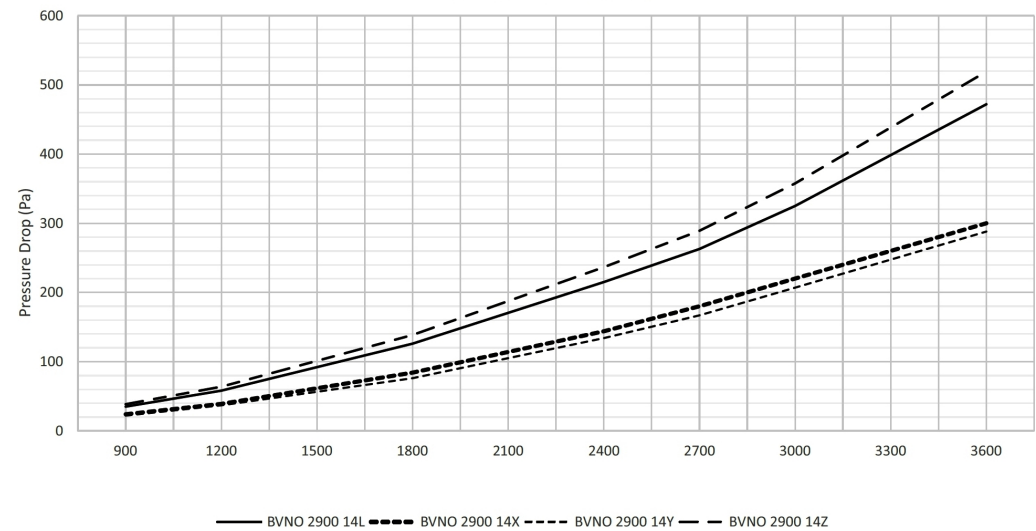
BVNO 2900 14L AND VARIANTS
